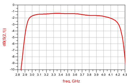
Insertion Loss VS Frequency (T A =25°C)
