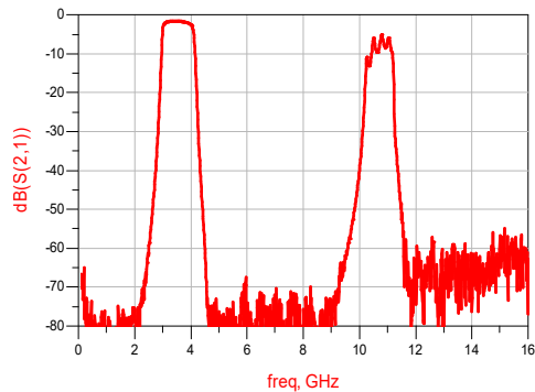
Broadband Insertion Loss VS Frequency ( T_A = 25^\circ\text{C} )
