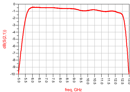
Insertion Loss & Return Loss VS Frequency (T A =25°C)
