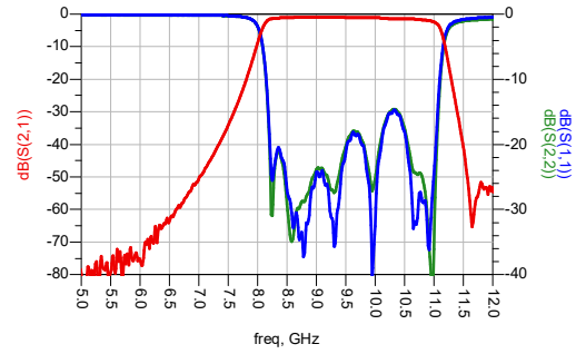
Broadband Insertion Loss VS Frequency ( T_A = 25^\circ\text{C} )
