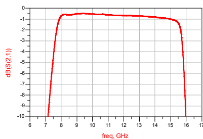
Insertion Loss VS Frequency ( T_A = 25^\circ\text{C} )
