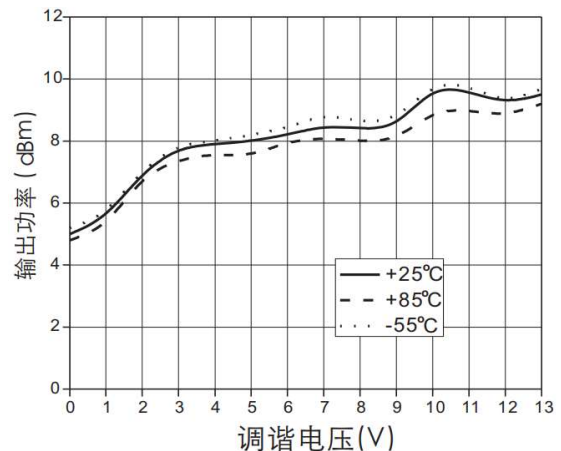
RFOUT/2 Output Power vs. Tuning Voltage Vcc=+5V
