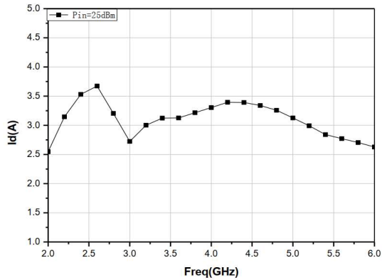
Drain Current
