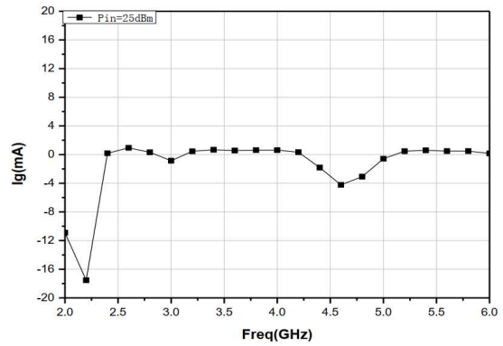
Gate Current
