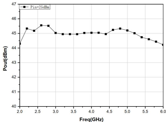
Output Power
