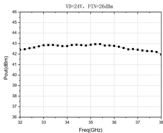
Output Power
