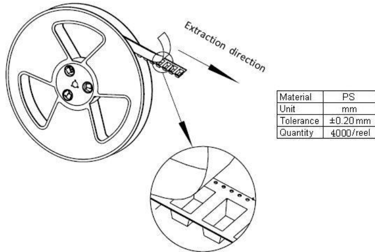
Outer Packing
