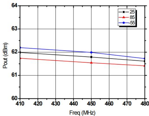
Pout, PAE&Freq.
