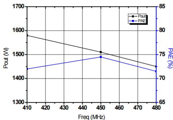
Pout, PAE&Freq.
