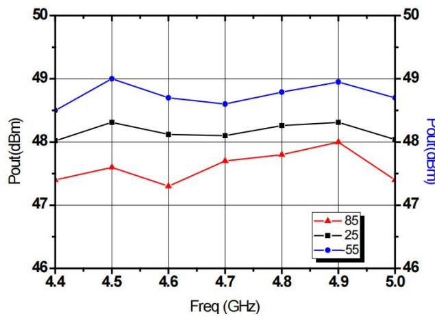
Pout&Freq. @ Different Temp.
