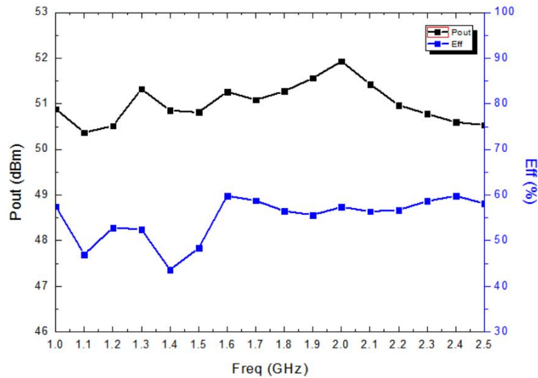
Pout、Eff&Freq.
