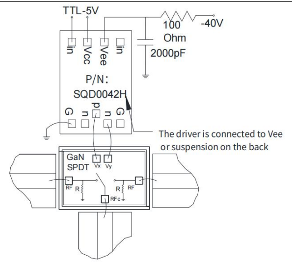
Assembly Diagram
