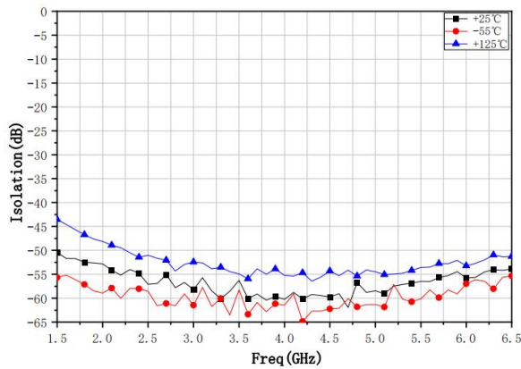
Isolation @ Different temperature
