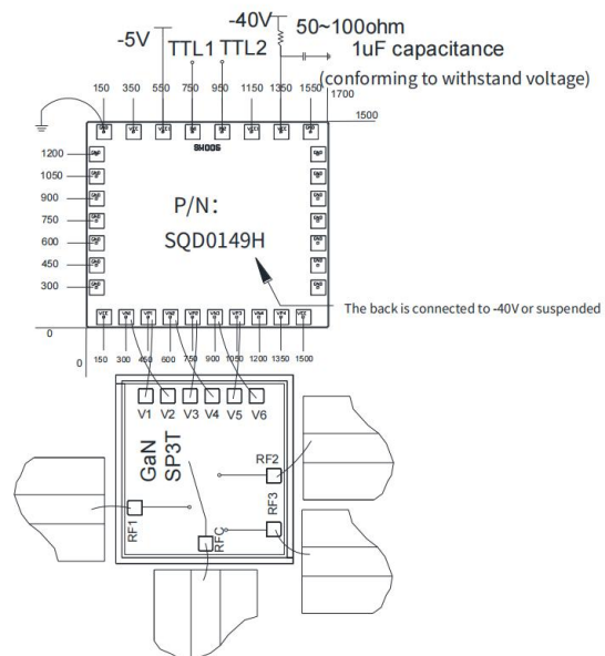
Assembly Diagram
