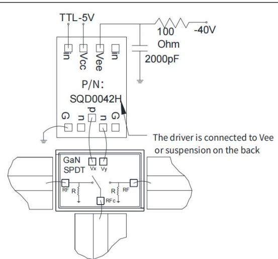
Assembly Diagram
