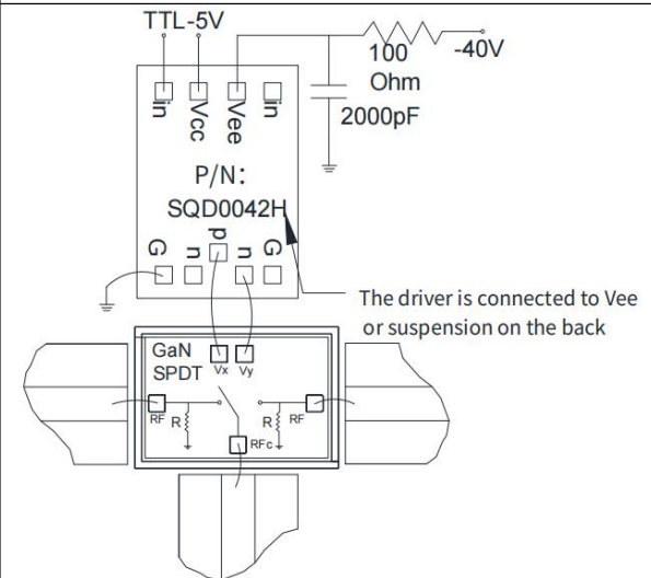
Assembly Diagram
