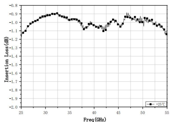
Insertion Loss
