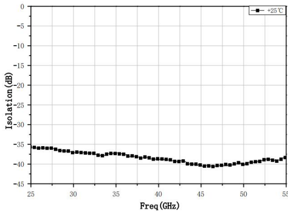
Isolation
