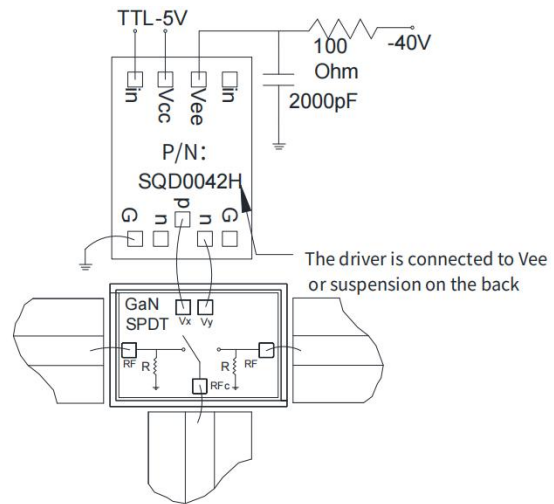
Assembly Diagram
