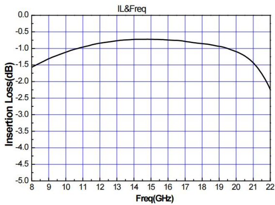
Insertion Loss
