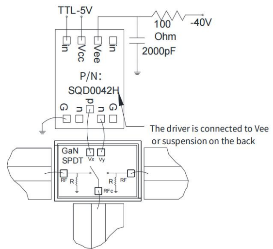
Assembly Diagram
