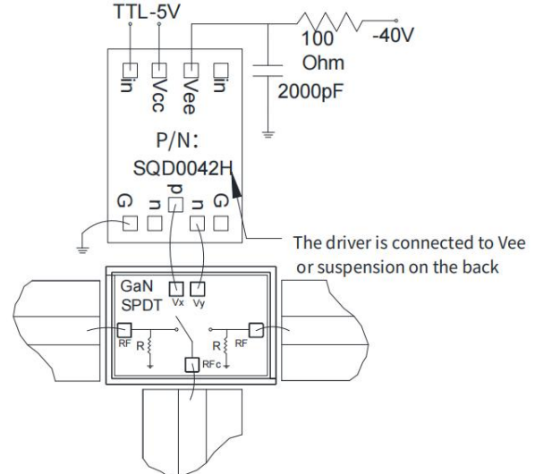
Assembly Diagram
