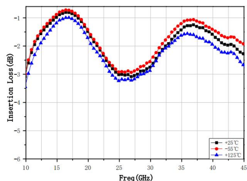
Insertion Loss @ Different temperature
