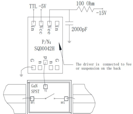
Assembly Diagram
