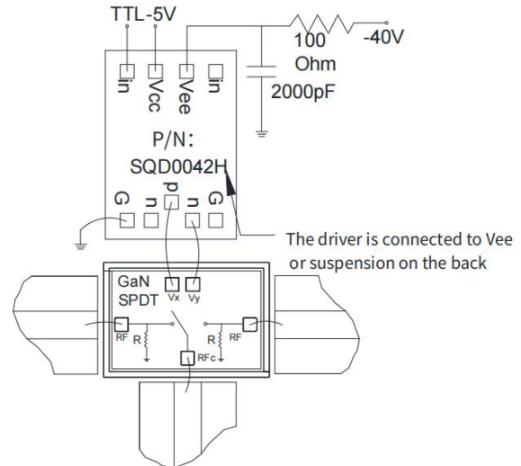
Assembly Diagram
