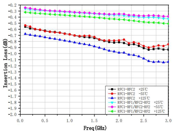
Insertion Loss @ Different temperature
