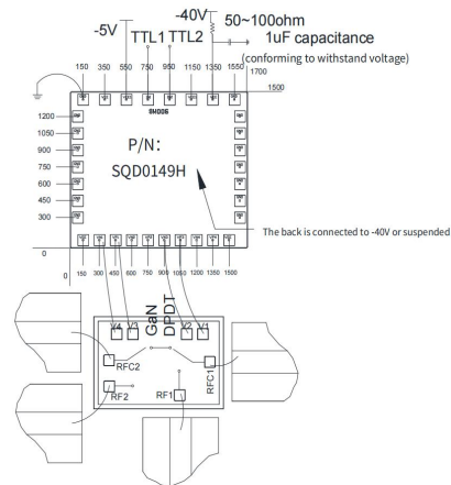
Assembly Diagram
