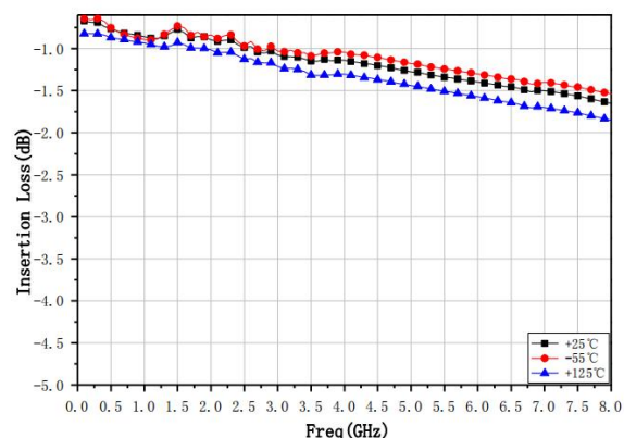
Insertion Loss @ Different temperature
