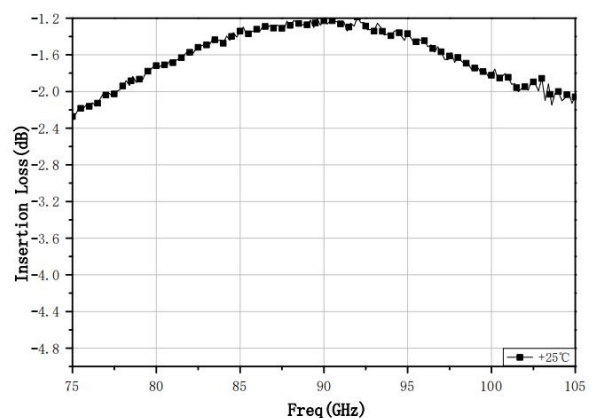
Insertion Loss
