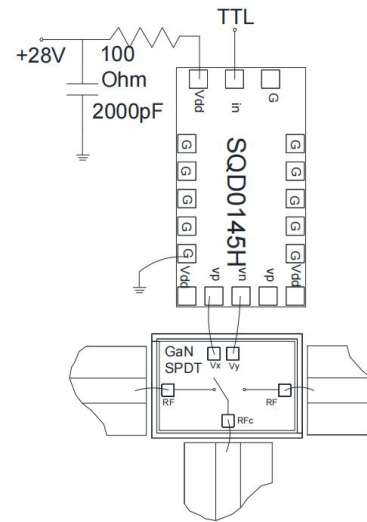
Assembly Diagram
