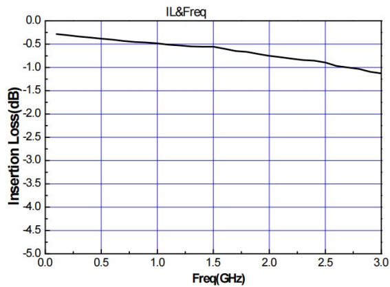
Insertion Loss
