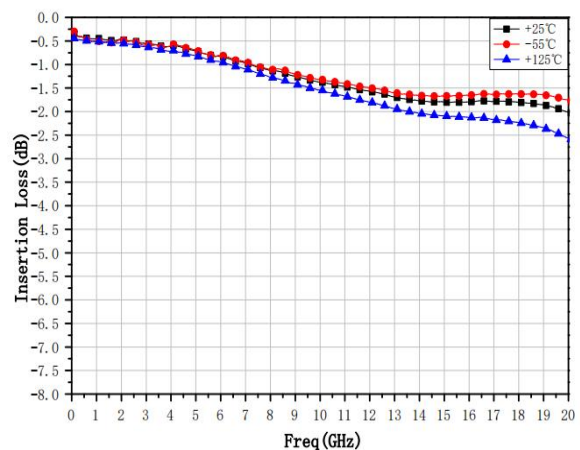
Insertion Loss @ Different temperature
