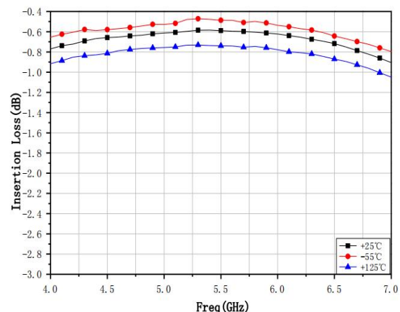
Insertion Loss @ Different temperature
