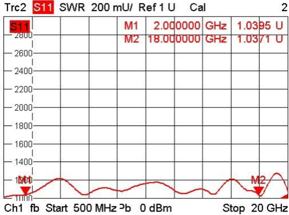
Coupling-Port VSWR
