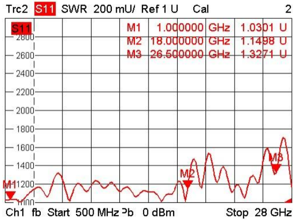
Coupling-Port VSWR
