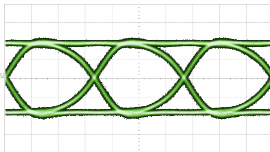
Figure 7: HL9491 56 Gbps PRBS 11, RF Input
