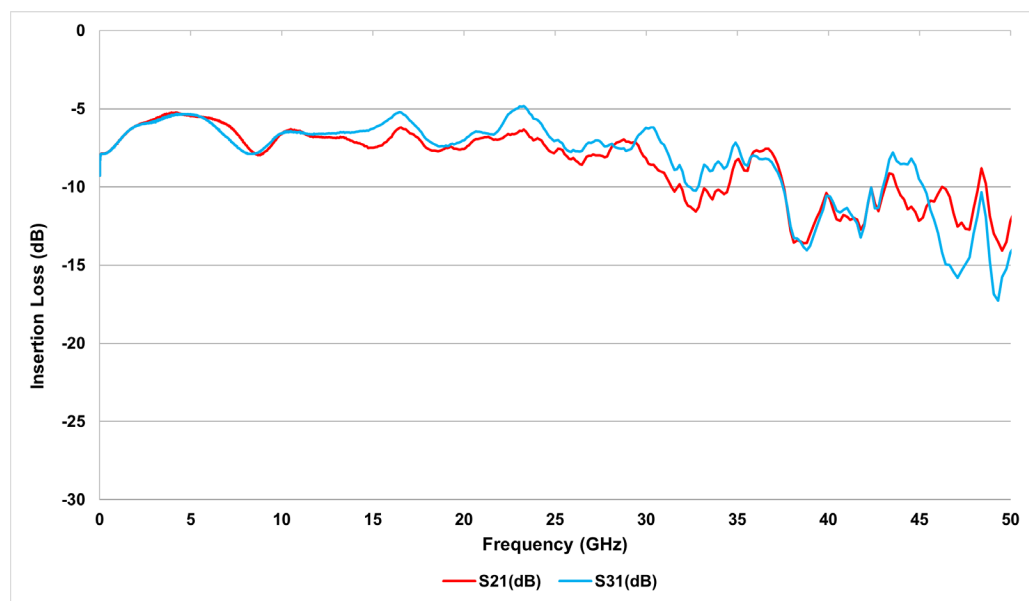
Figure 2: HL9492 Single-ended Insertion Loss - linear scale
