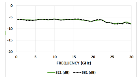
Typical HL7071 Insertion Loss
