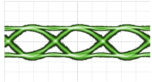
56 Gbps NRZ pattern on the Thru Out port of HL9467-JPJ; see also Figs. 13-24
