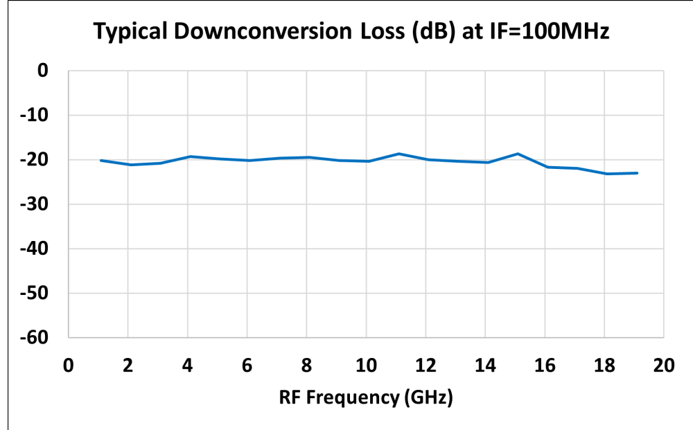
Figure 1: HL9334 Conversion Loss Measured at LO = 2 GHz, IF = 100 MHz, -10 dBm RF Input Power
