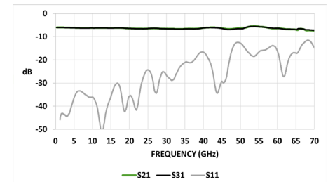
Typical HL9487 Insertion and Return Loss
