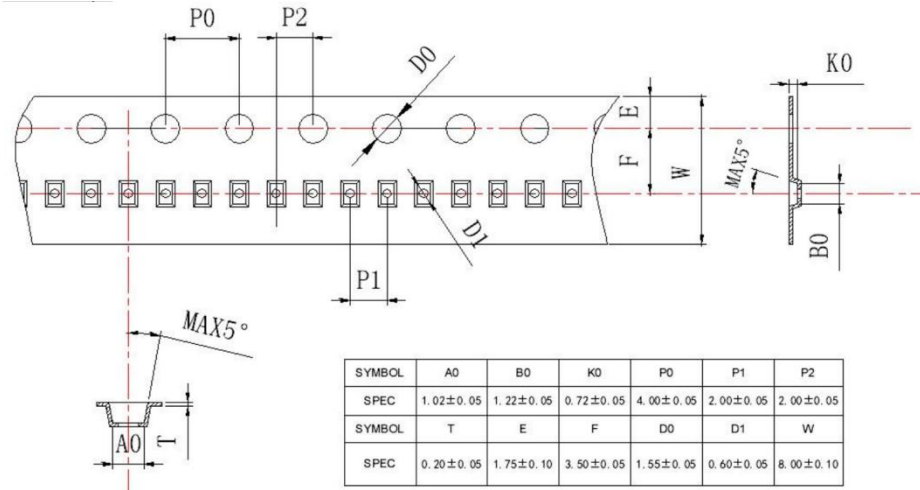
Carrier Tape
